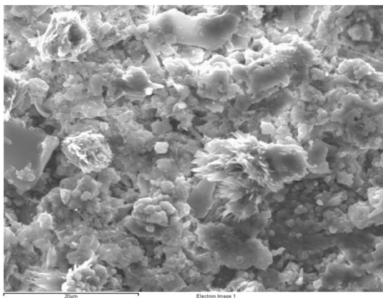
Figure 4. Anderson Dock nickel SEM image of the formation of cuprite and atacamite crystals as corrosion products. Atacamite mineral formation is shown by the platy crystals and cuprite formation is shown in the granular crystals 5 . Scale bar represents 20 \mu\text{m} .
