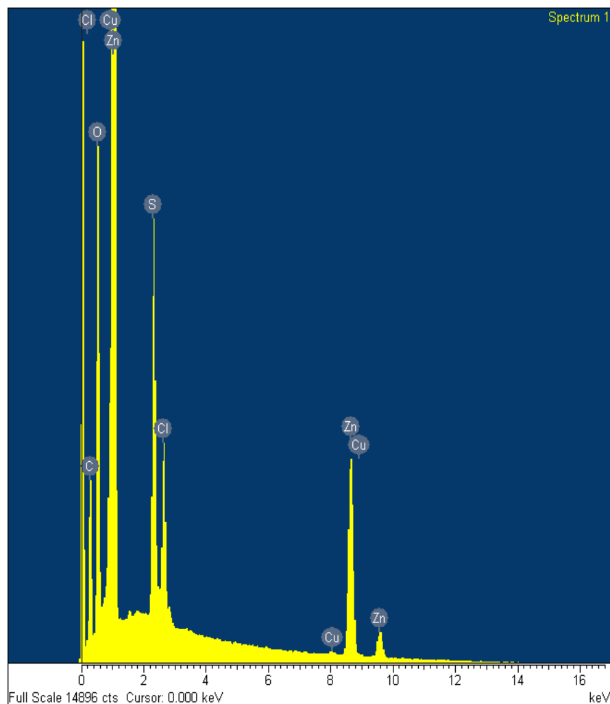
Figure 5. EDS spectrum showing the chemical composition of the Emerald Isle Marsh young penny. ESD spectrums provided elemental atomic and weight percentages at specific points (1 \mu m) on the coin samples.
