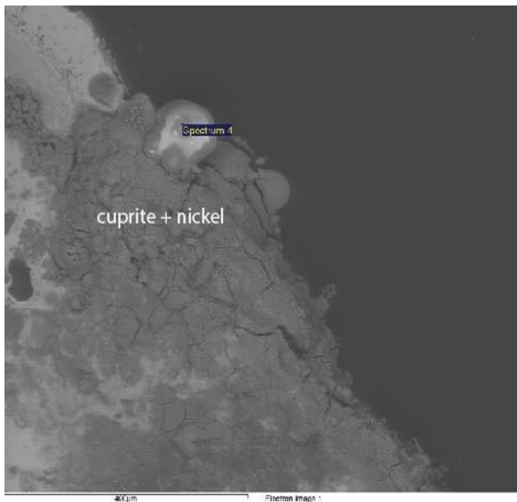
Figure 7. SEM image of the Bent Creek dime shows the development of cuprite minerals near the surface, with intermittent nickel remaining present; however, no nickel corrosion minerals were found to have developed. Scale bar represents 400 \mu\text{m} .
