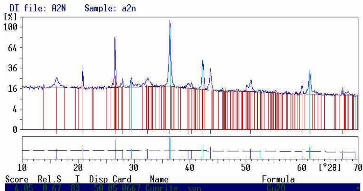
Figure 3. XRD spectrum for Anderson Dock nickel showing strong peak matches for the presence of cuprite (aqua blue markers) in the sample.
