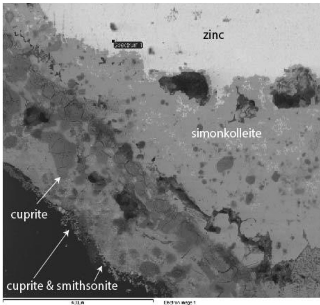
Figure 6. SEM image of the Emerald Isle Marsh young penny showing the phase development of copper and zinc minerals: zinc core, phasing to simonkolleite, cuprite, and a thin outer layer of cuprite and smithsonite. Scale bar represents 400 \mu\text{m} .
