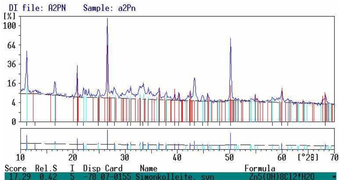
Figure 2. XRD spectrum for Anderson Dock young penny shows a strong match for the presence of simonkolleite minerals in the sample. Aqua blue markers show peaks for simonkolleite, and other colors represent other phases, such as cuprite and zinc.
