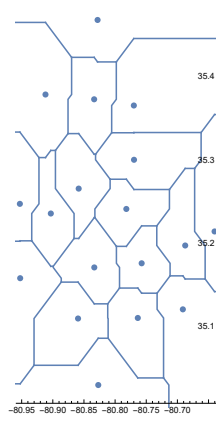
FIGURE 3.2. A Taxicab Voronoi diagram of CMS public high schools.
